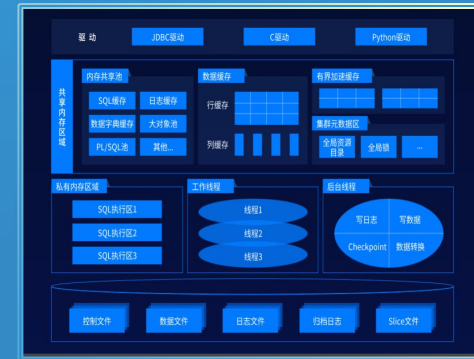
Yashan Database system
